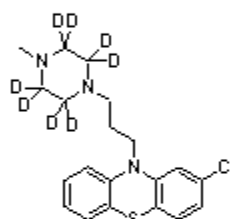
Prochlorperazine-D8
