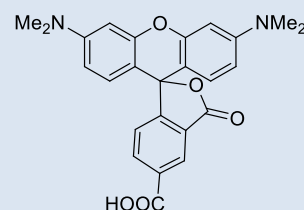
6-TAMRA (6-Carboxytetramethylrhodamine)
