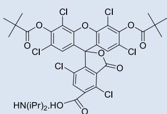
5-Hex-Cl-FAM-COOH.NH(iPr) 2
