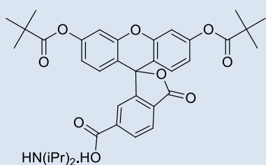
6-FAM-COOH.NH(iPr) 2
