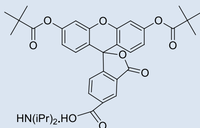
5-FAM-COOH.NH(iPr) 2
