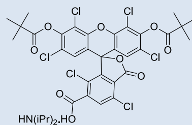
6-Hex-Cl-FAM-COOH.NH(iPr) 2
