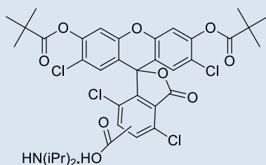
5/6-TET-FAM-COOH.NH(iPr) 2
